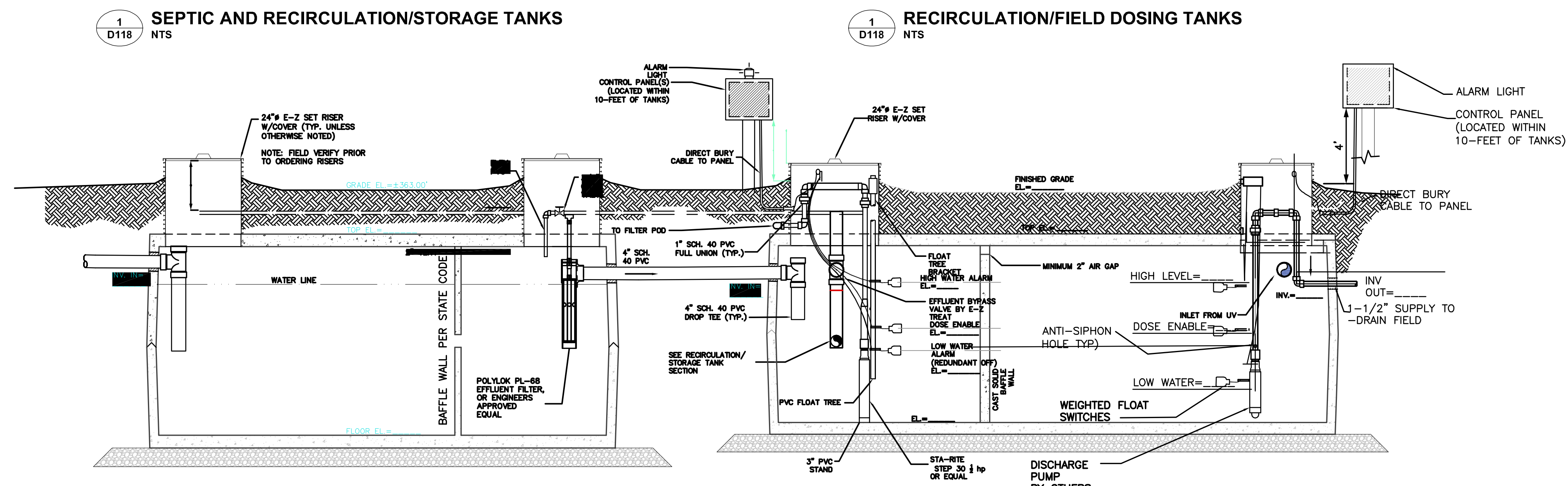
D D118 NTS SEPTIC AND RECIRCULATION/STORAGE TANK SECTIONS
